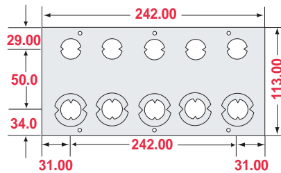
Knock-out Panel CC-01, 02, 03, 04
