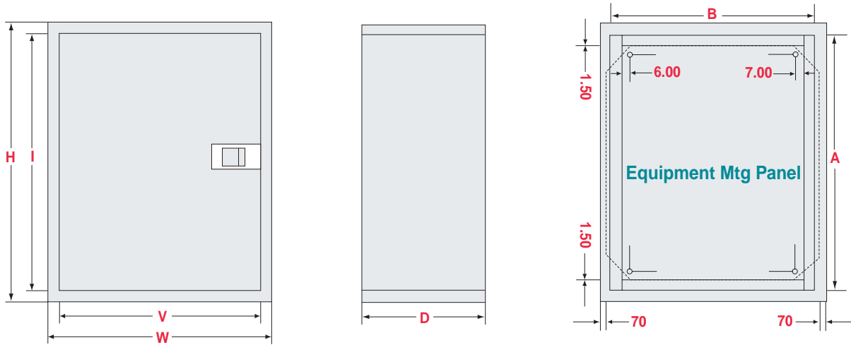
Knock-out Panel CC-01, 02, 03, 04
